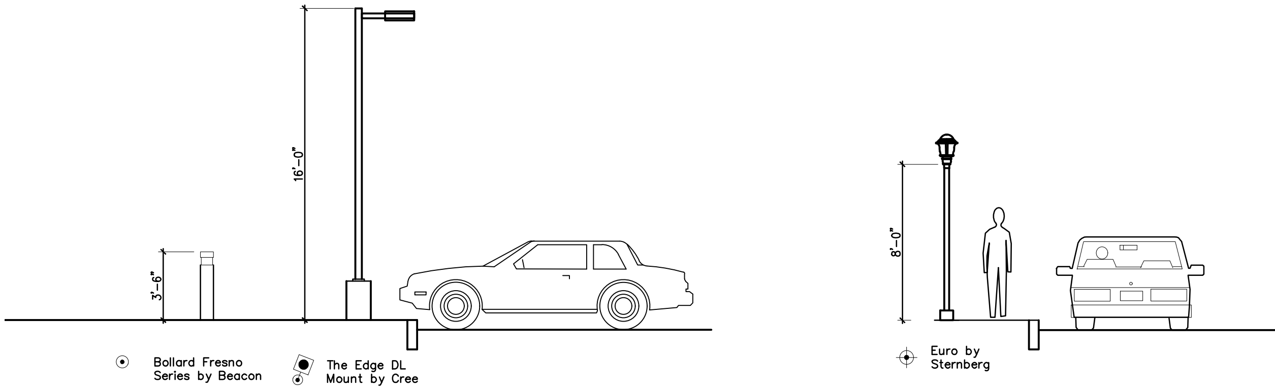
5 SITE LIGHT ELEVATION SCALE: NTS
