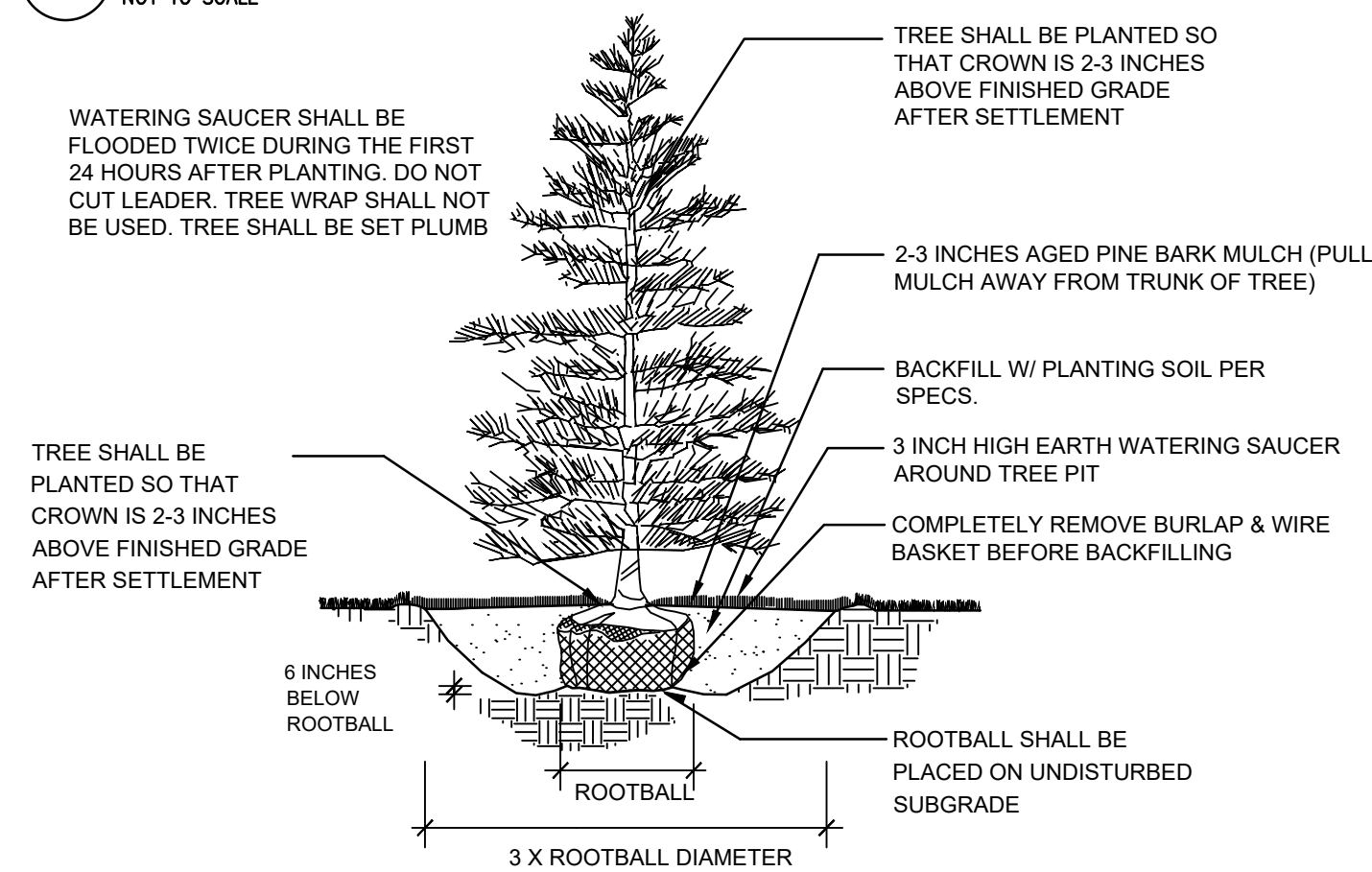
EVERGREEN TREE PLANTING NOT TO SCALE
