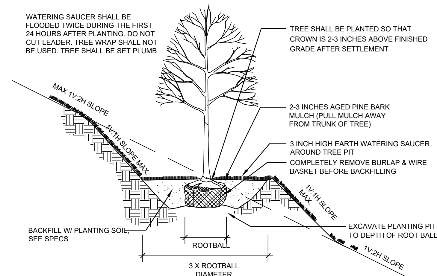
DECIDUOUS TREE PLANTING (SLOPE) NOT TO SCALE
