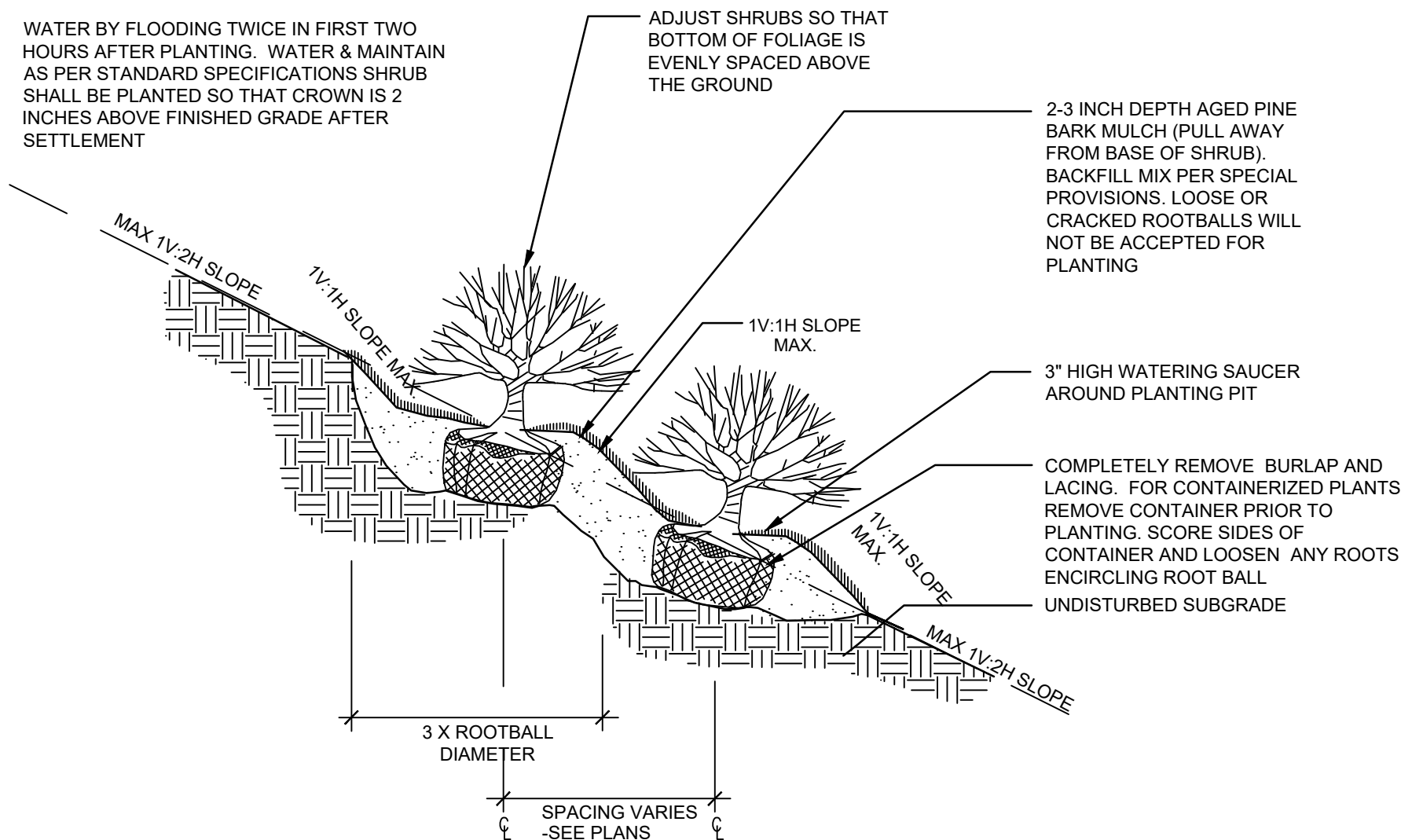
CONTAINERIZED SHRUB PLANTING (SLOPE) DETAIL NOT TO SCALE
