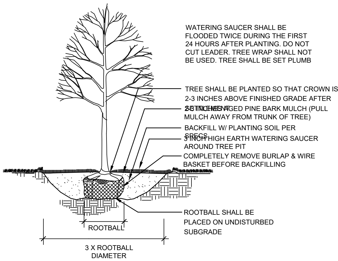
DECIDUOUS TREE PLANTING NOT TO SCALE
