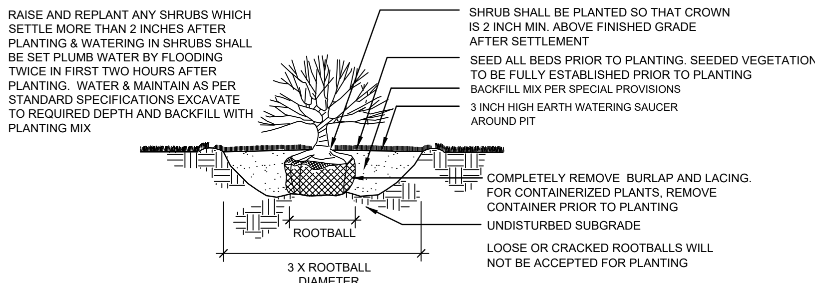
SHRUB PLANTING NOT TO SCALE
